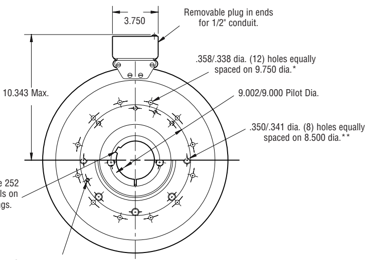
ARMATURE VIEW
