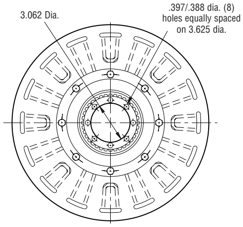
ARMATURE VIEW
