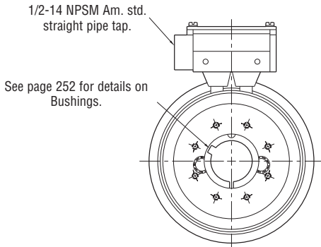
COLLECTOR RING VIEW
