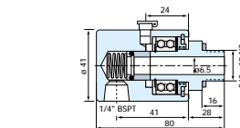
1/4" ROTO Coupling part No 40067-730
