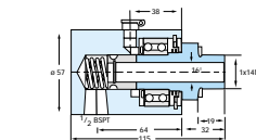
1" ROTO Coupling part No 24181-040
