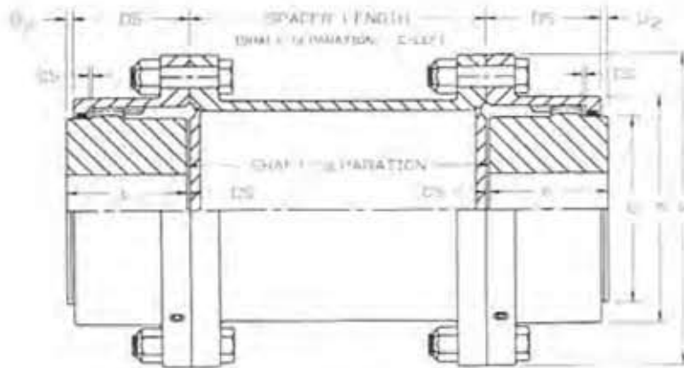
Full Flex Limited End Float (L.E.F.) Spacer Coupling
