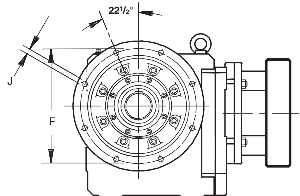
Drawing for Units K913-K1014F
