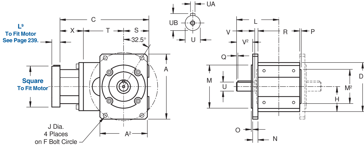
Drawing for Units KL102VF — KL202VF
