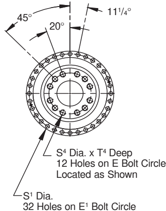
PHQA9/PHQA10 OUTPUT SIDE
