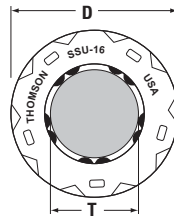
Super Smart Ball Bushing Bearings (Closed Type) and 60 Case® LinearRace® Shafting (Dimensions in inches)
