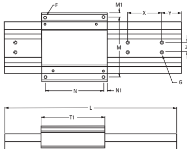
Dual Shaft Rail Linear Guide with Integrated Full Length Carriage
