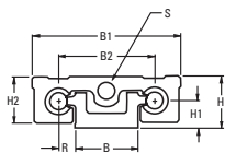
2DA XX 00A Rail Cross Section
