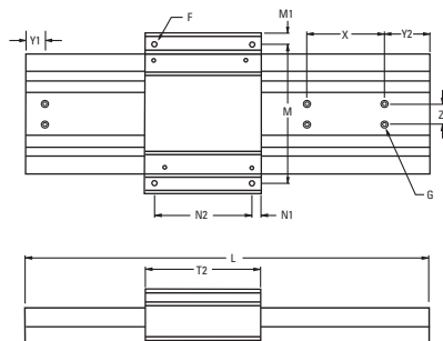
Dual Shaft Rail Linear Guide with Integrated Short Length Carriage
